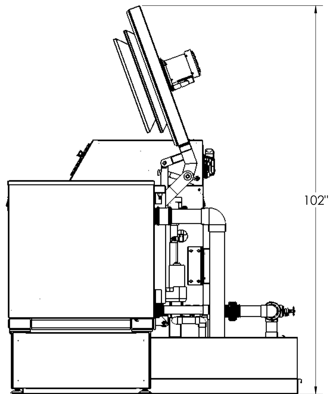
Lid Shown @ 70° Open
